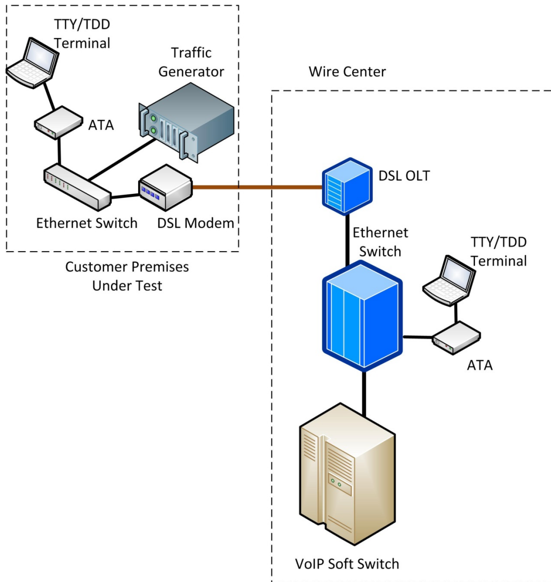
Figure 7 – TTY/TDD Test Setup
