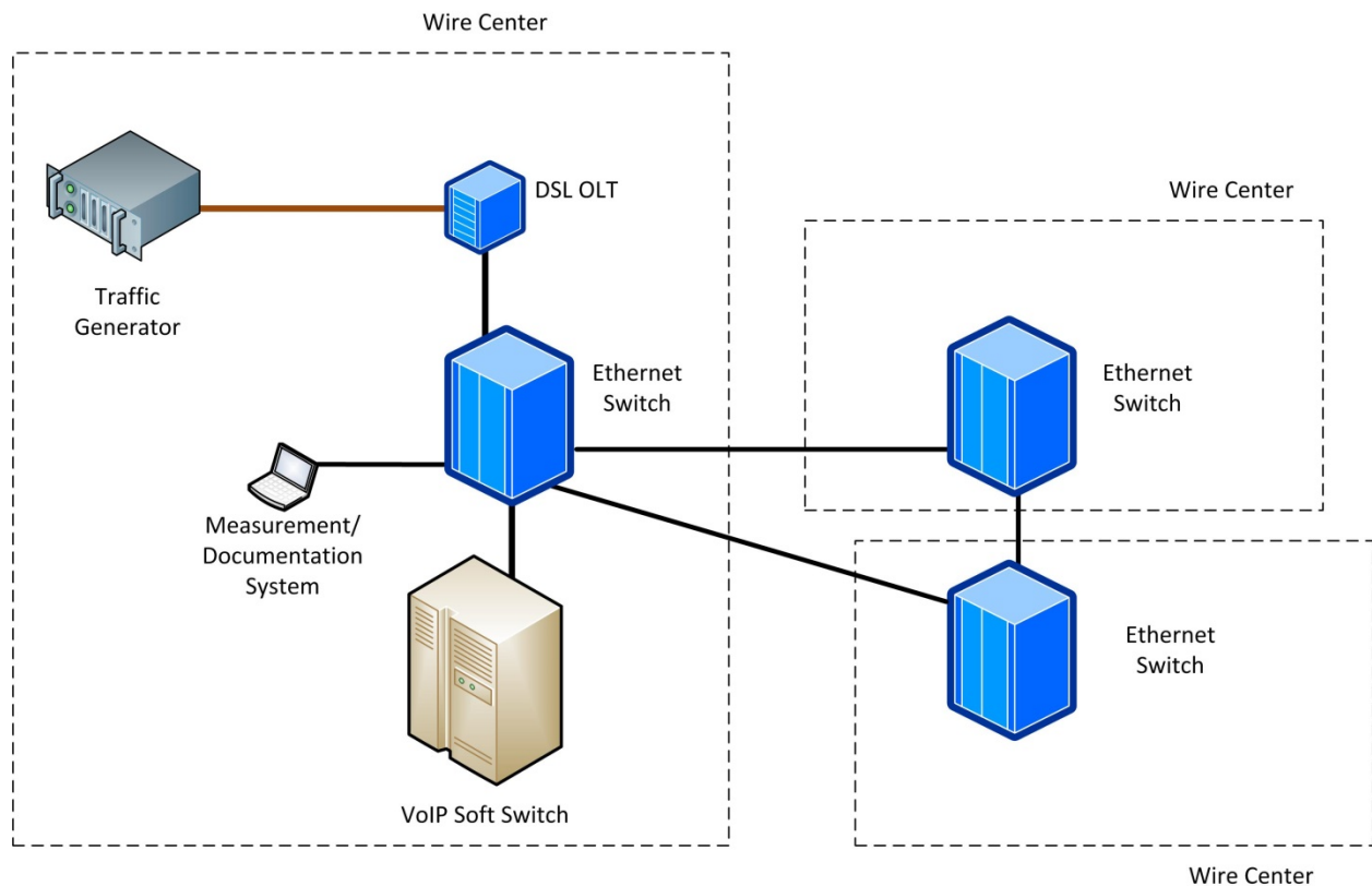
Figure 3 – Stress Test Configuration
