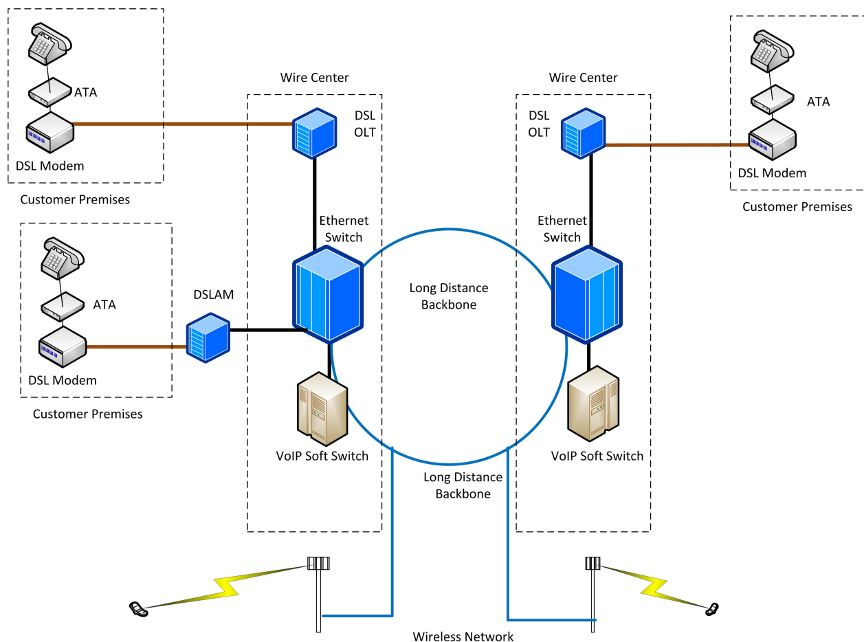
Figure 2 – Telephone in an IP Environment
