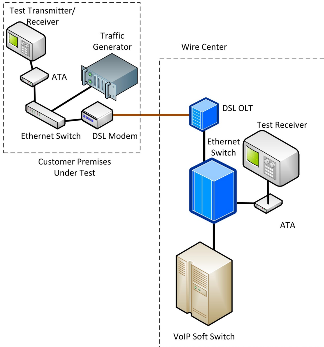
Figure 4 – Field Test from Test Transmitter at Customer Premises
