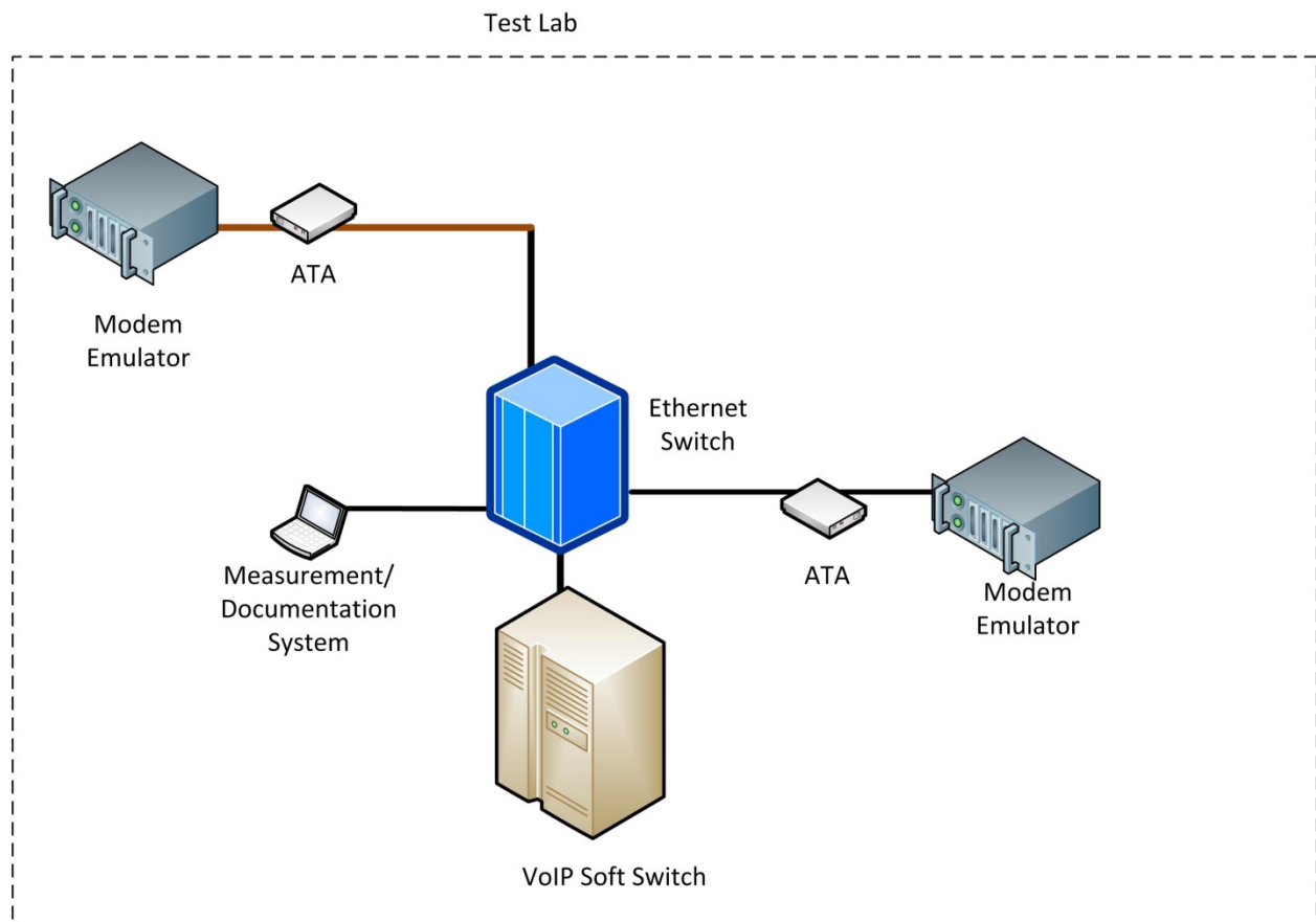
Figure 6 – Interoperability Test Setup
