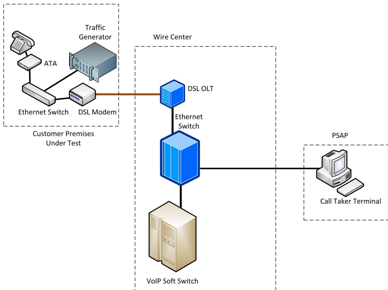
Figure 8 – 9-1-1 Test Configuration
