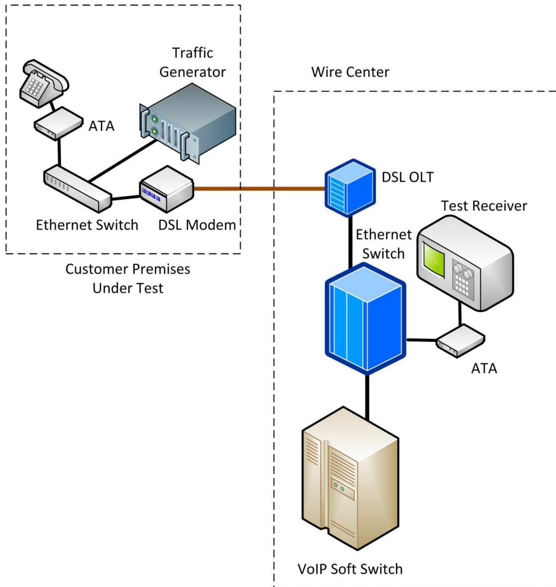
Figure 5 – Field Test from Telephone at Customer Premises
