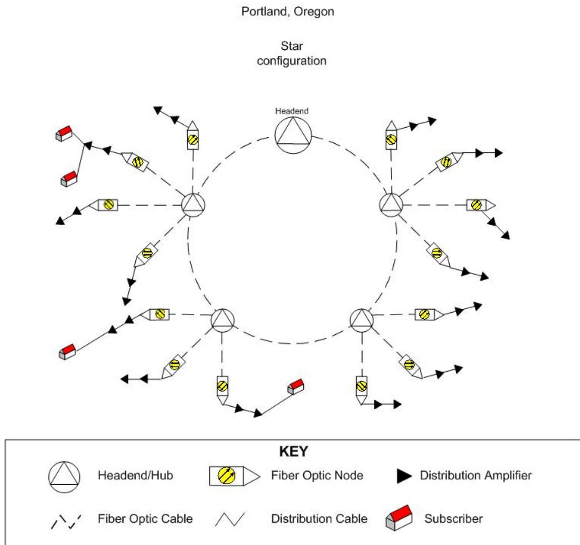
Figure 2: Portland Network Architecture
