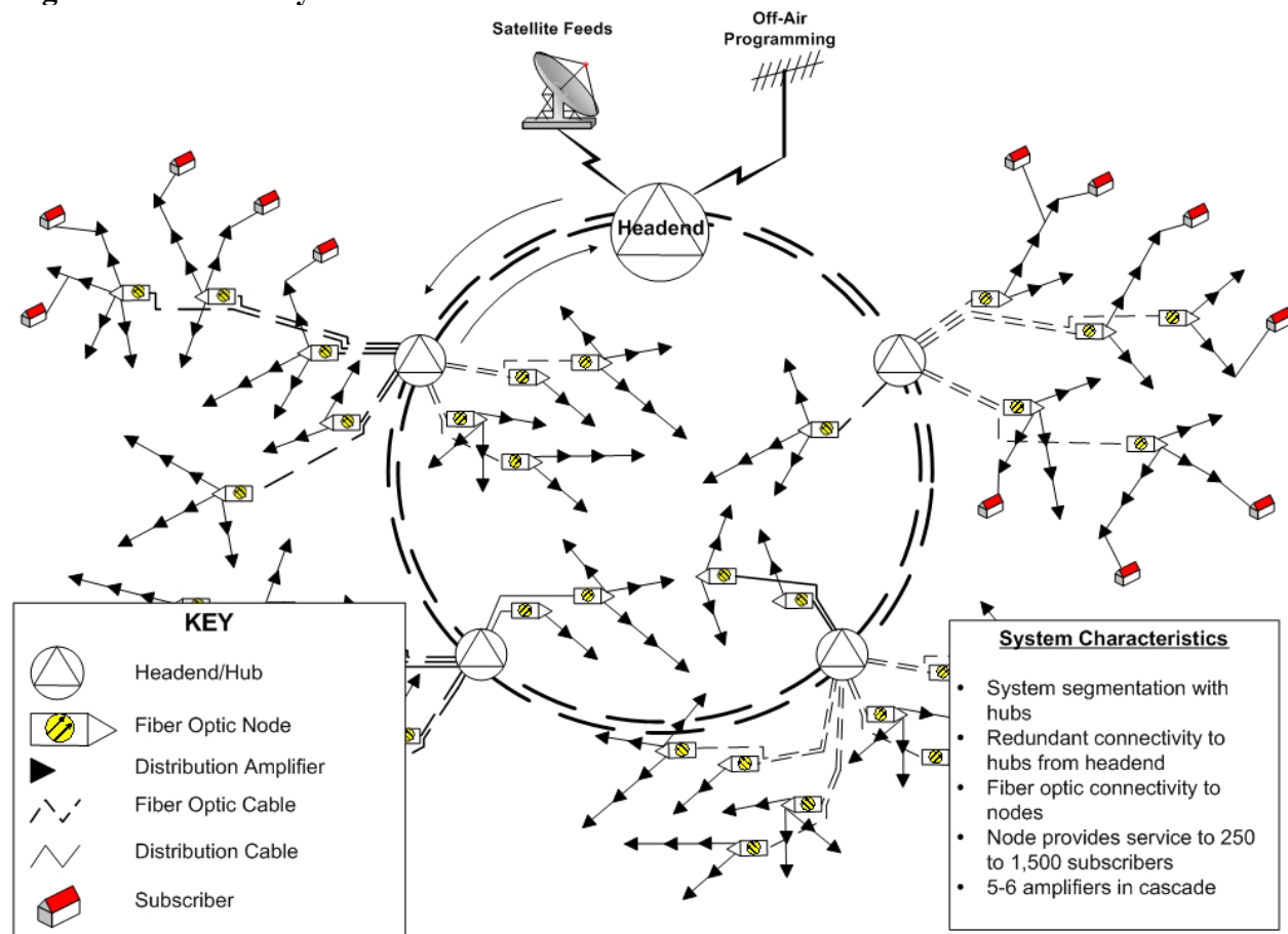
Figure 1: Modern Hybrid Fiber/Coaxial Architecture
