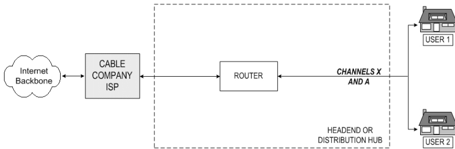
Figure 3: Summary Diagram of Four Models for Cable Modem Service Single-ISP Standard
