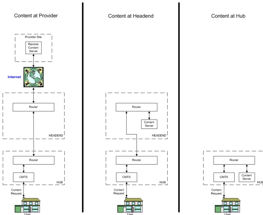
Figure 5: Locating Content Locally
