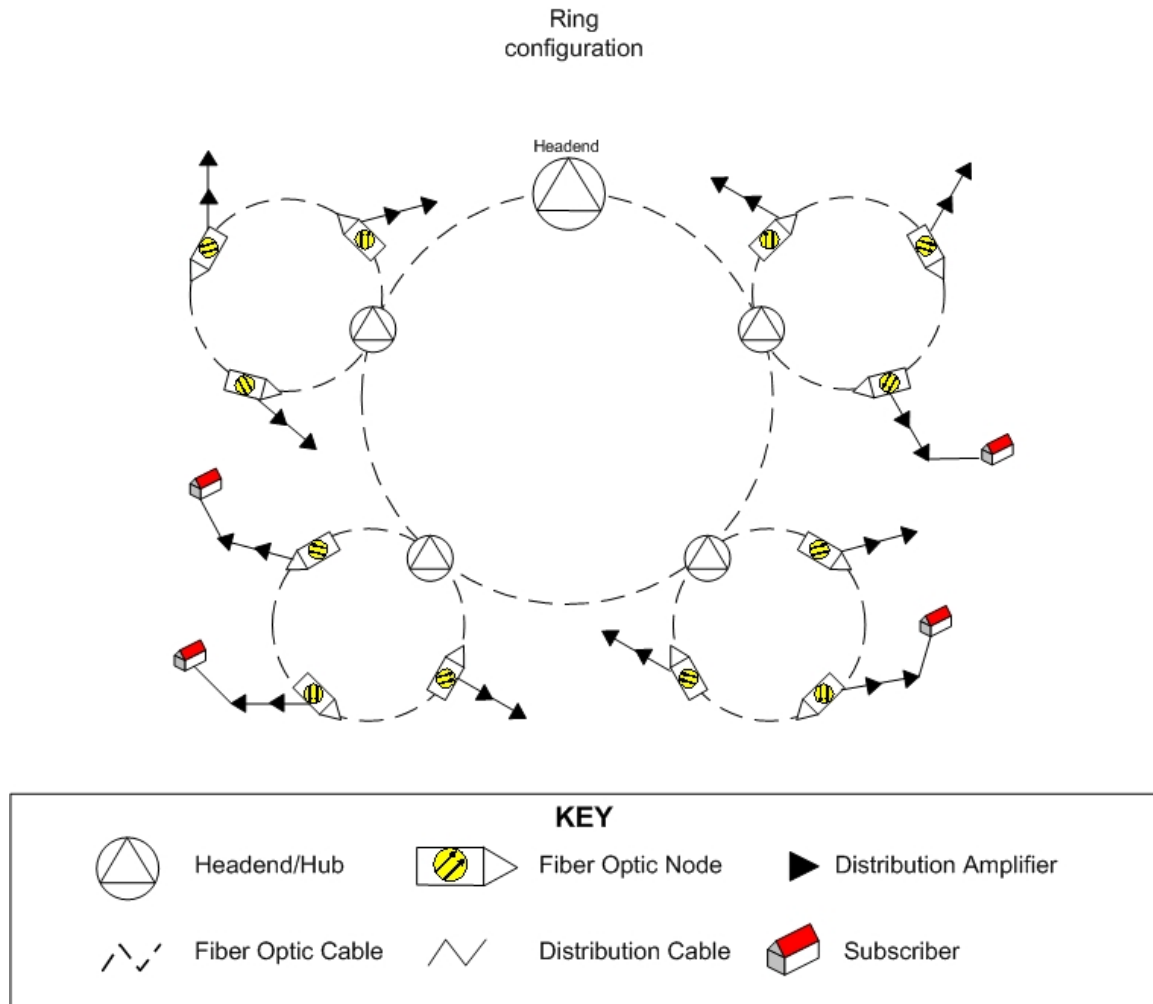
Figure 1: Click! Network Architecture Tacoma, Washington
