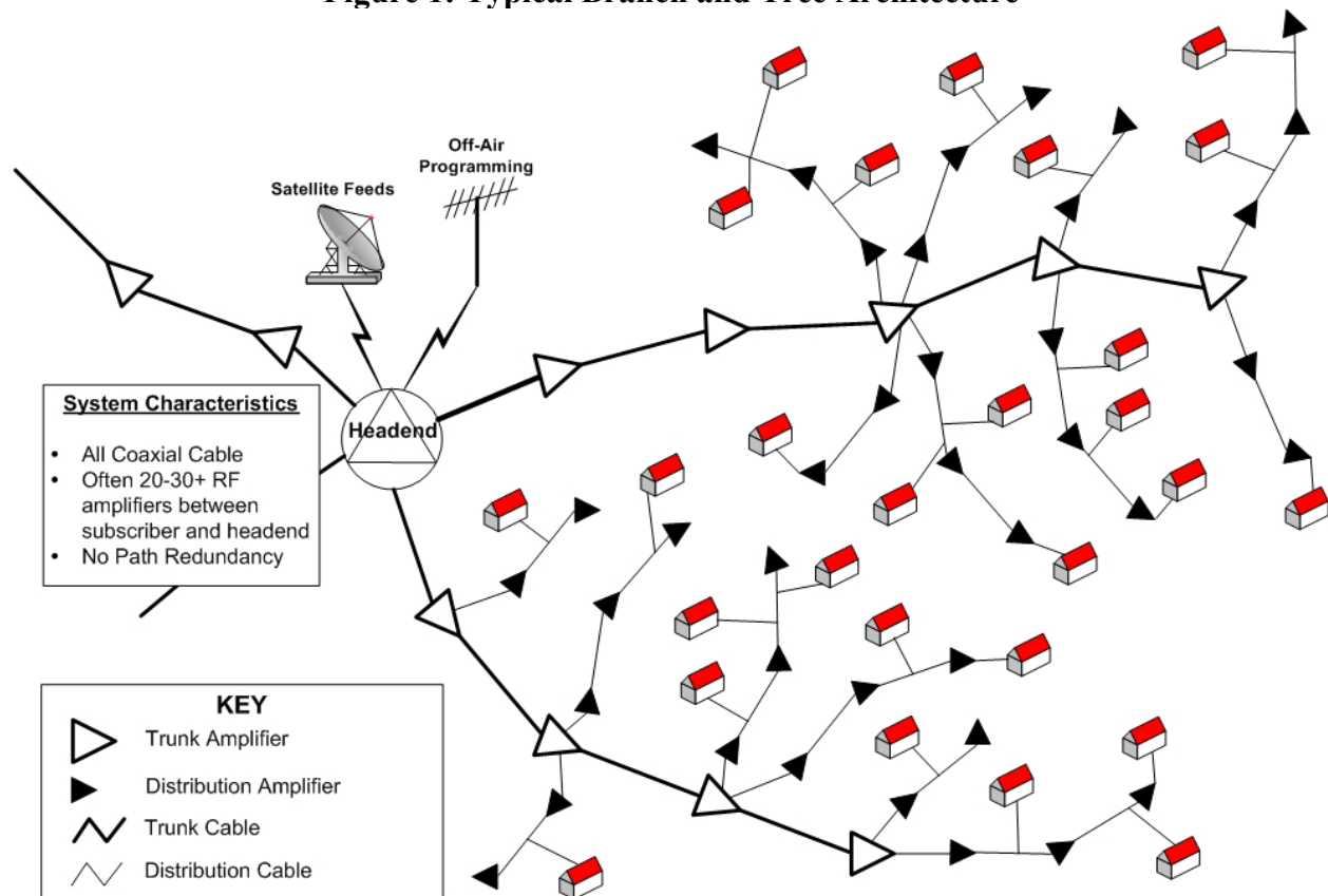
Figure 1: Typical Branch and Tree Architecture
