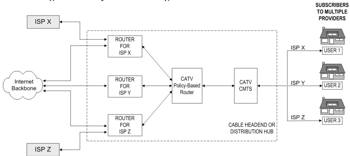
Figure 7: Policy-Based Routing with ISP Co-Location at Headend
