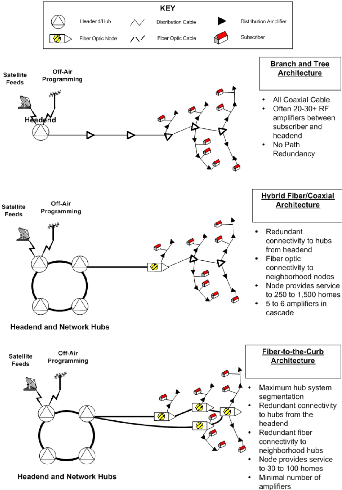
Figure 1: Summary Diagram of Three Categories of Cable Architecture
