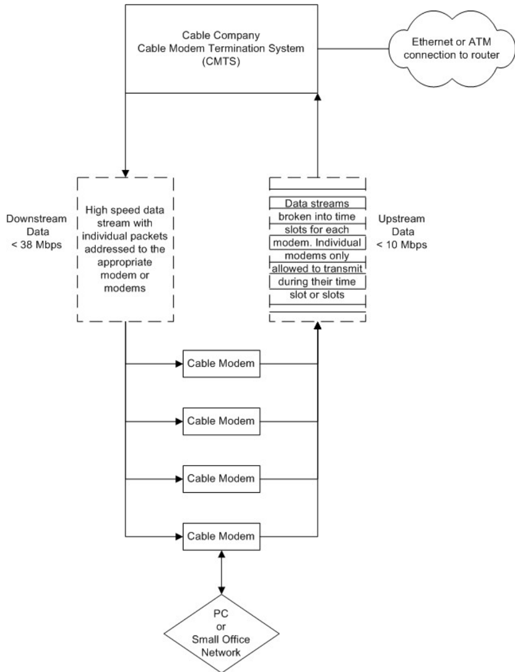
Figure 3: Cable Modem Transmission
