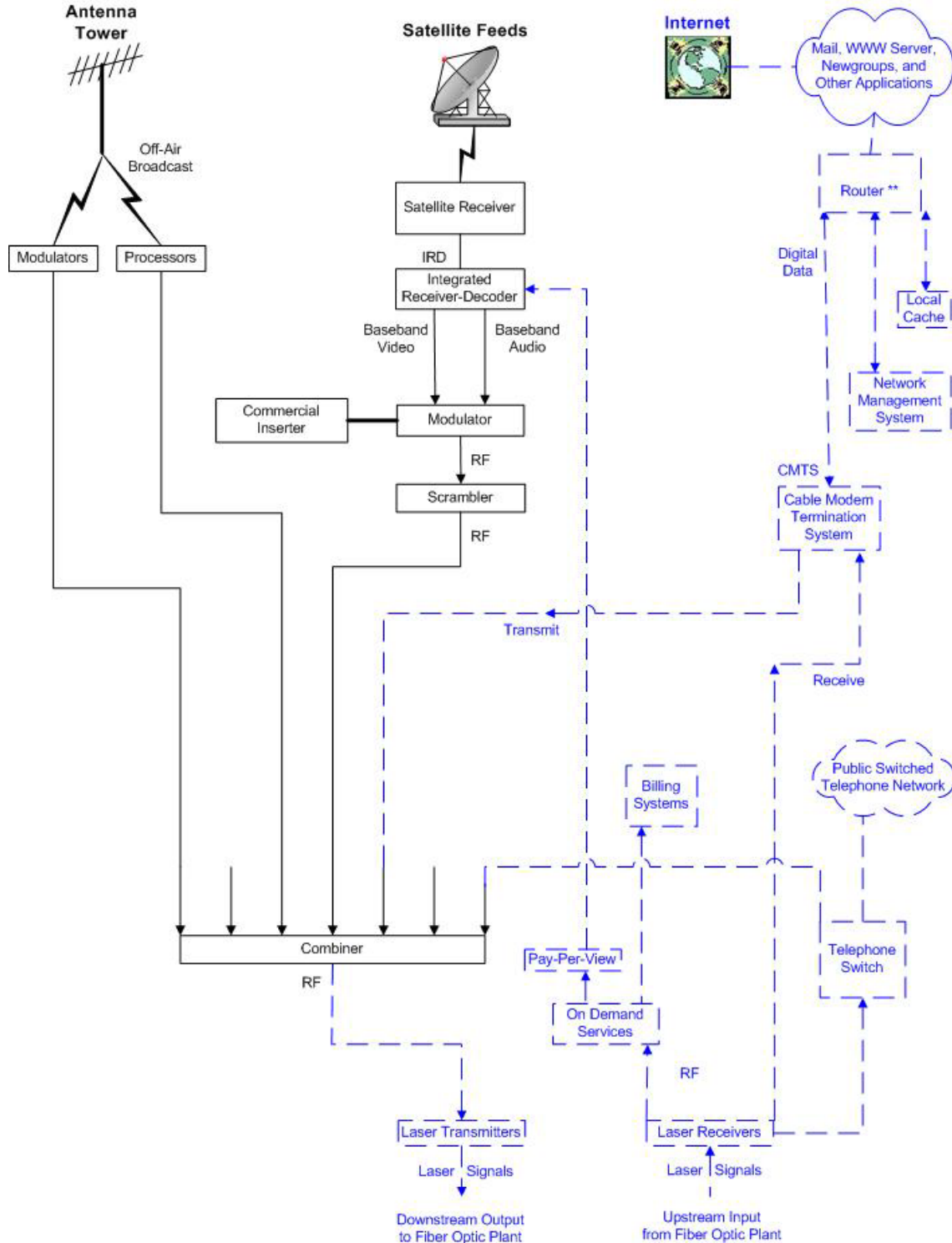
Figure 2: Hybrid Fiber/Coaxial Headend*
