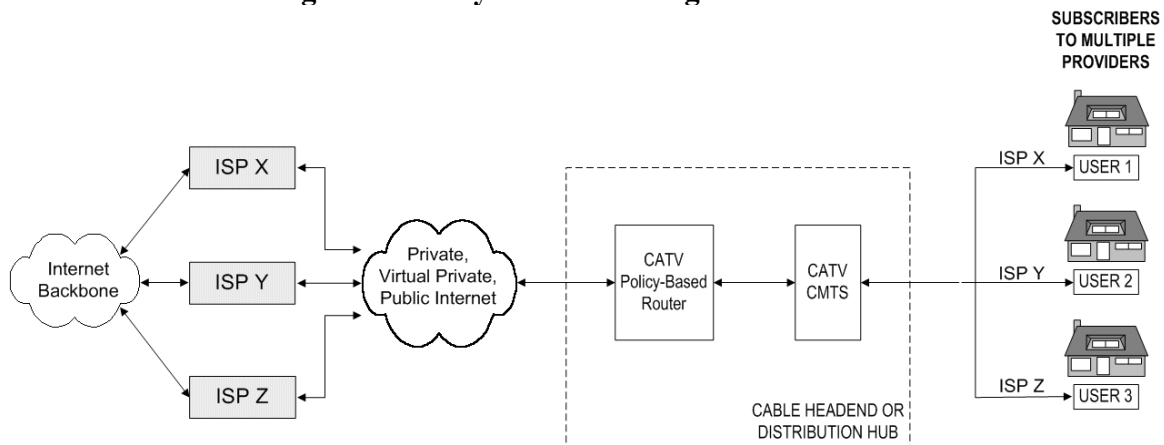
Figure 8: Policy-Based Routing Over Internet
