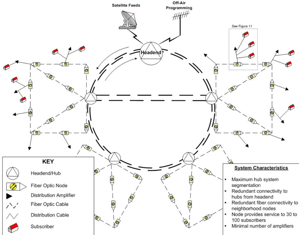
Figure 1: Fiber-to-the-Curb Architecture
