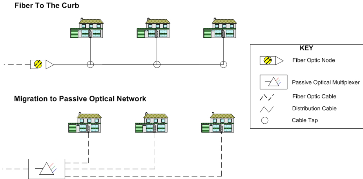
Figure 3: Migration from Fiber-to-the-Curb to Passive Optical Network (from Figure 2)
