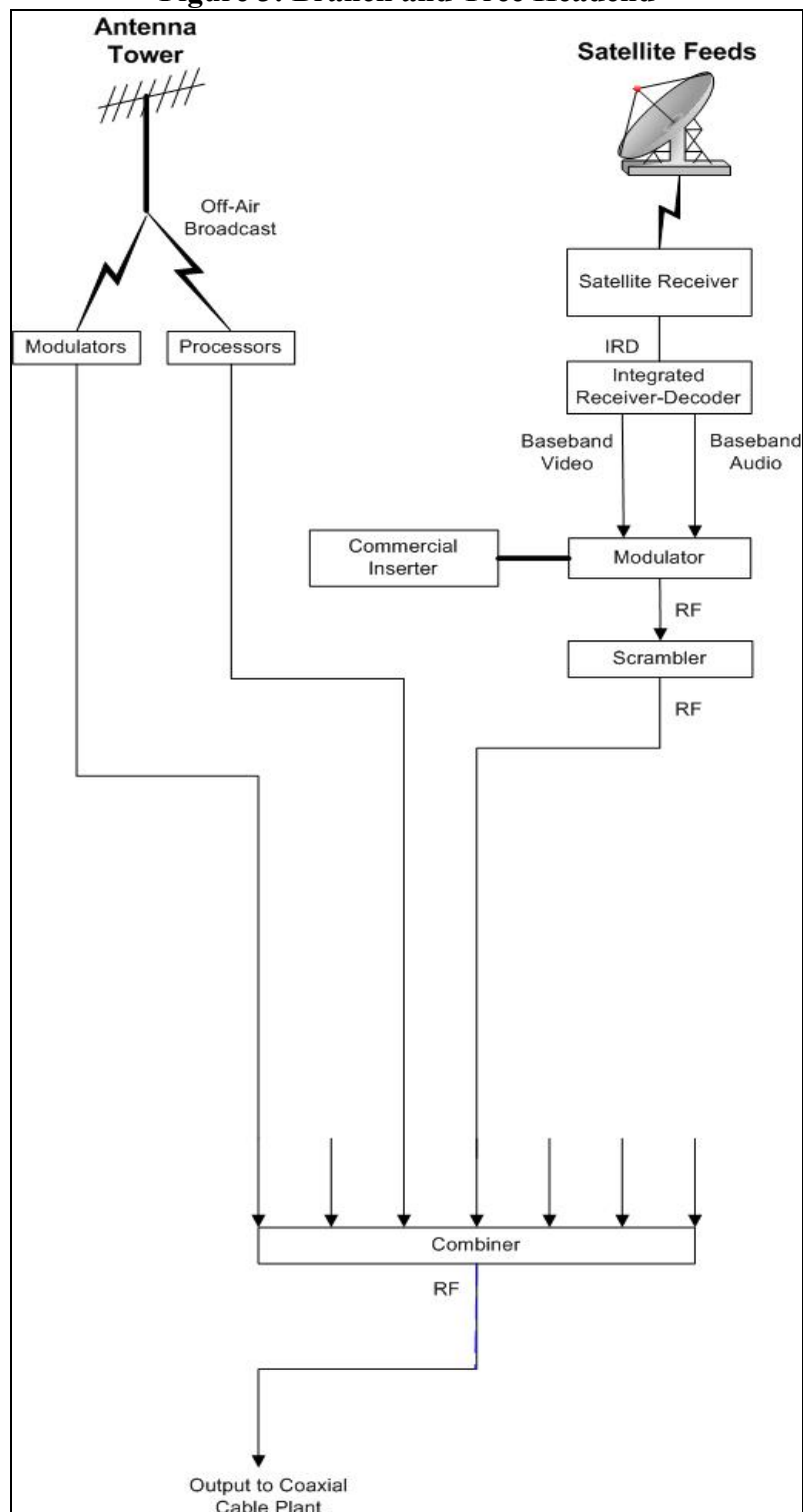
Figure 3: Branch and Tree Headend
