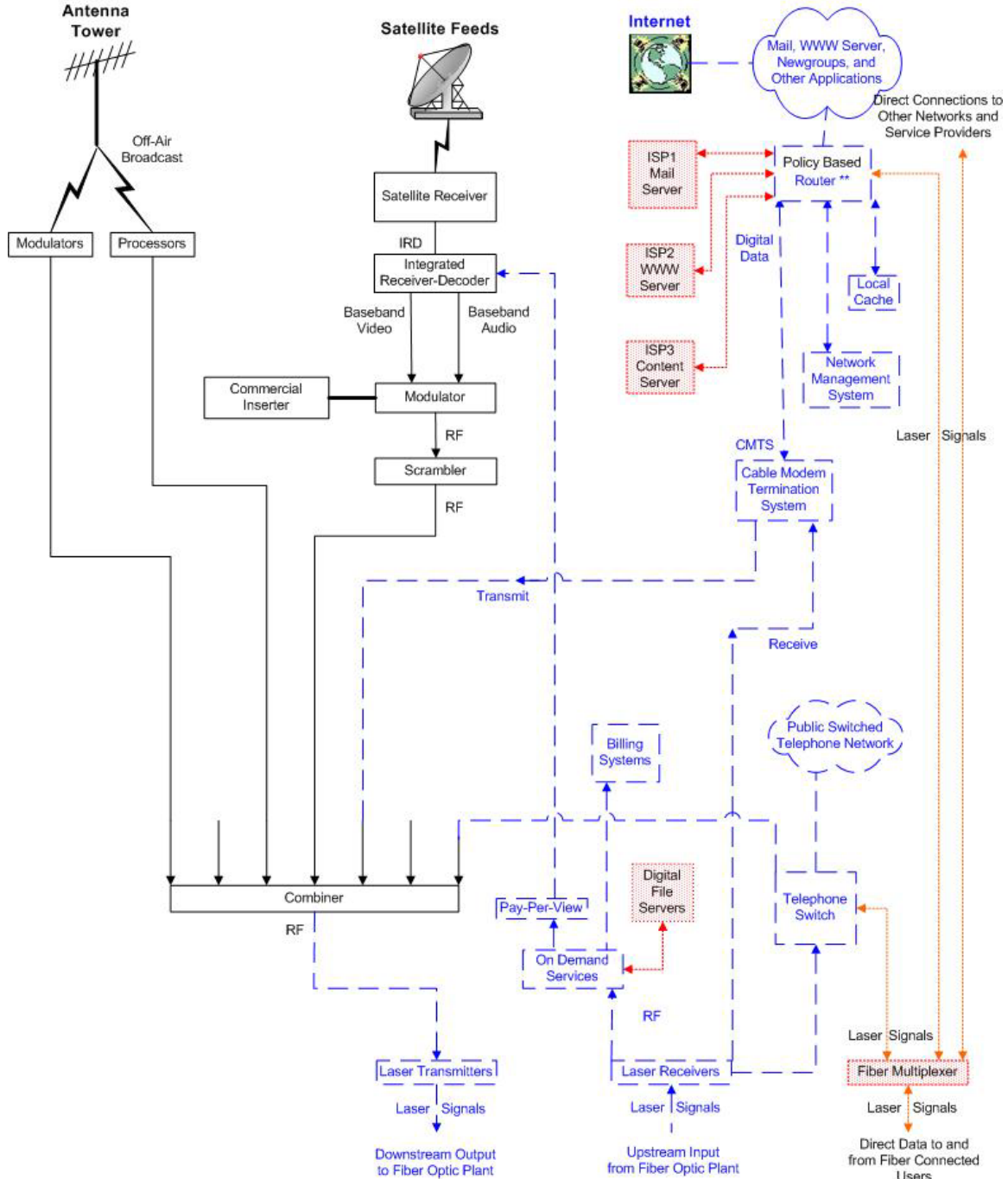
Figure 2: Fiber-to-the-Curb Headend*
